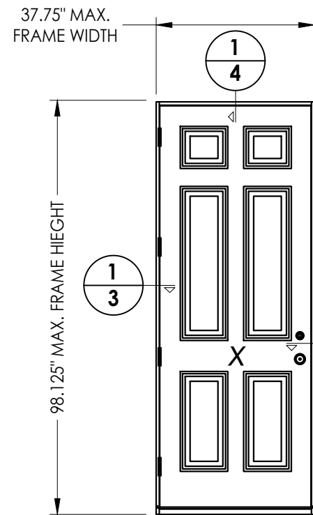
SINGLE DOOR (Shown with opaque door)
